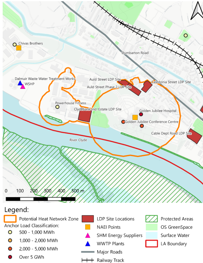
Figure 0—7 Golden Jubilee Hospital Heat Network Zone
